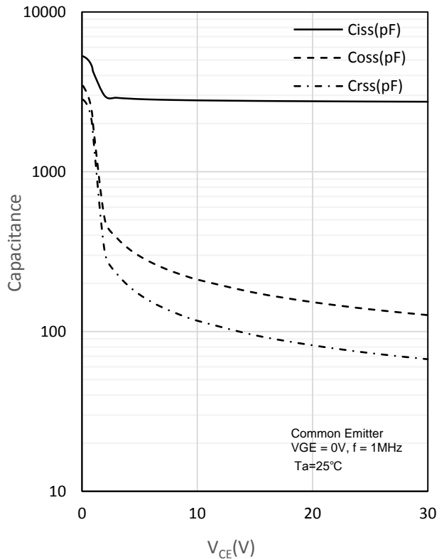
Fig. 12 Capacitance characteristics
